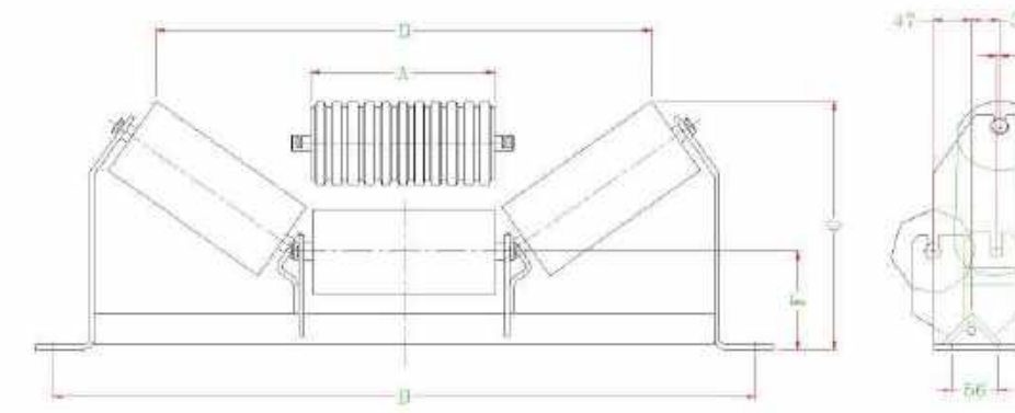
SERIES LS/RS 3 ROLL TROUGH IDLERS-OFFSET 114 DIAMETER
